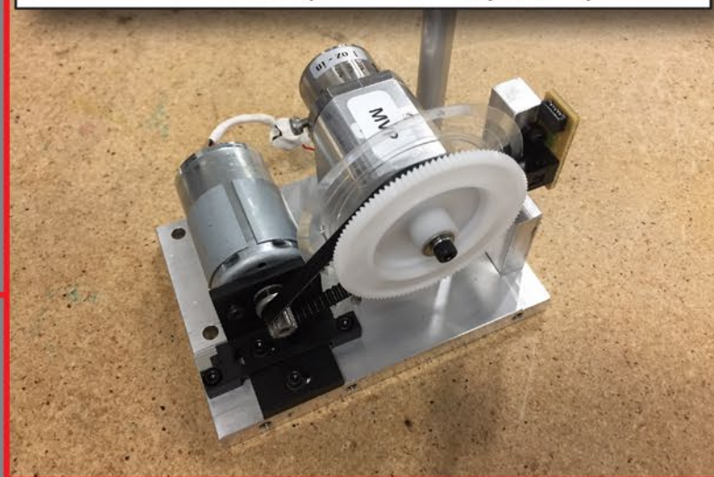
PT-1320-A006 | Drive Assy Complete
